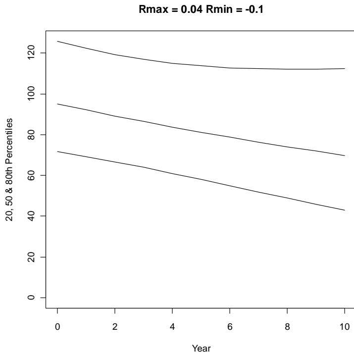
Figure 2. Cetacean example w/ CV= 0.35. Lower 20 th percentile decreases at ~5.0% per year.
