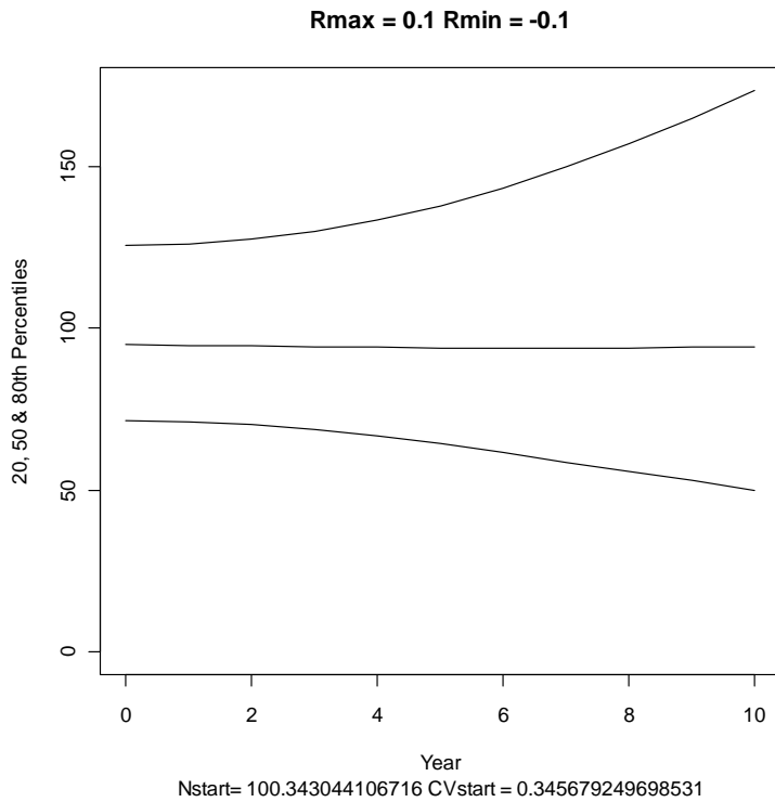
Figure 4. Symmetrical growth rate \sim R(-0.1,+0.1) w/ CV= 0.35: Lower 20 th percentile decreases at \sim 3.5\% per year.
