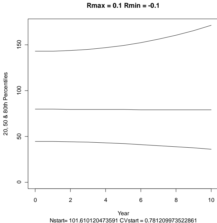
Figure 5. Symmetrical growth rate \sim R(-0.1,+0.1) w/ CV= 0.80: Lower 20 th percentile decreases at \sim 2.1\% per year.
