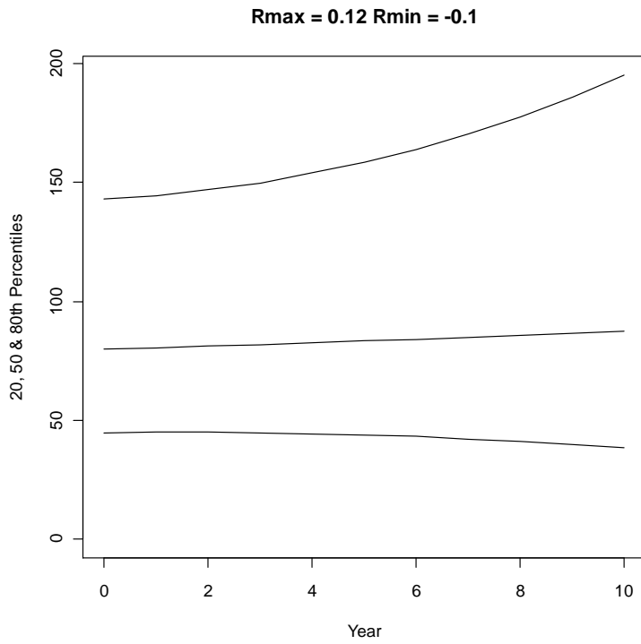
Figure 3. Pinniped example w/ CV= 0.80. Lower 20 th percentile decreases at ~1.5% per year.
